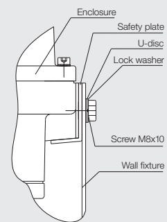
Wall mounting
